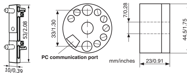
DIN-rail adapter
